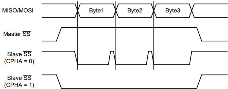
Figure 16- 5 CPHA/SS 时序
