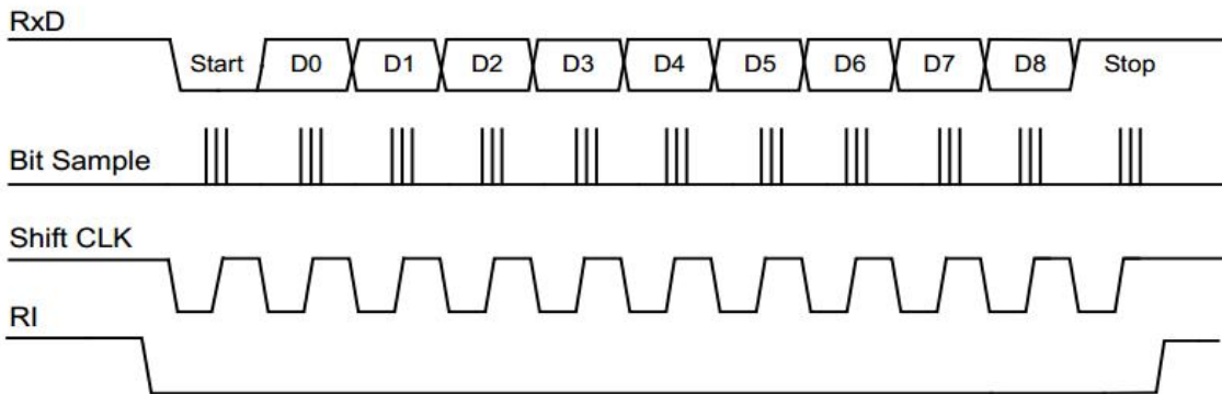
Figure 14-5 Receive Timing of Mode 2
