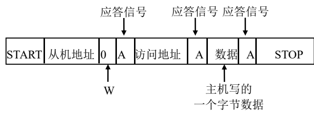
Figure 17-7 主机向从机写数据
