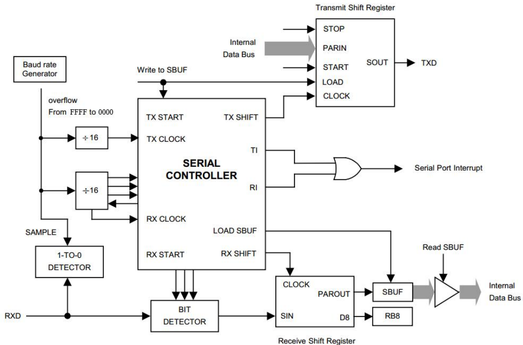
Figure 15-1 Receive Shift Register
