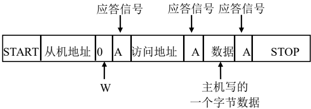
Figure 17-7 主机向从机写数据
