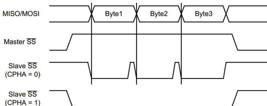
Figure 16-5 CPHA/SS 时序
