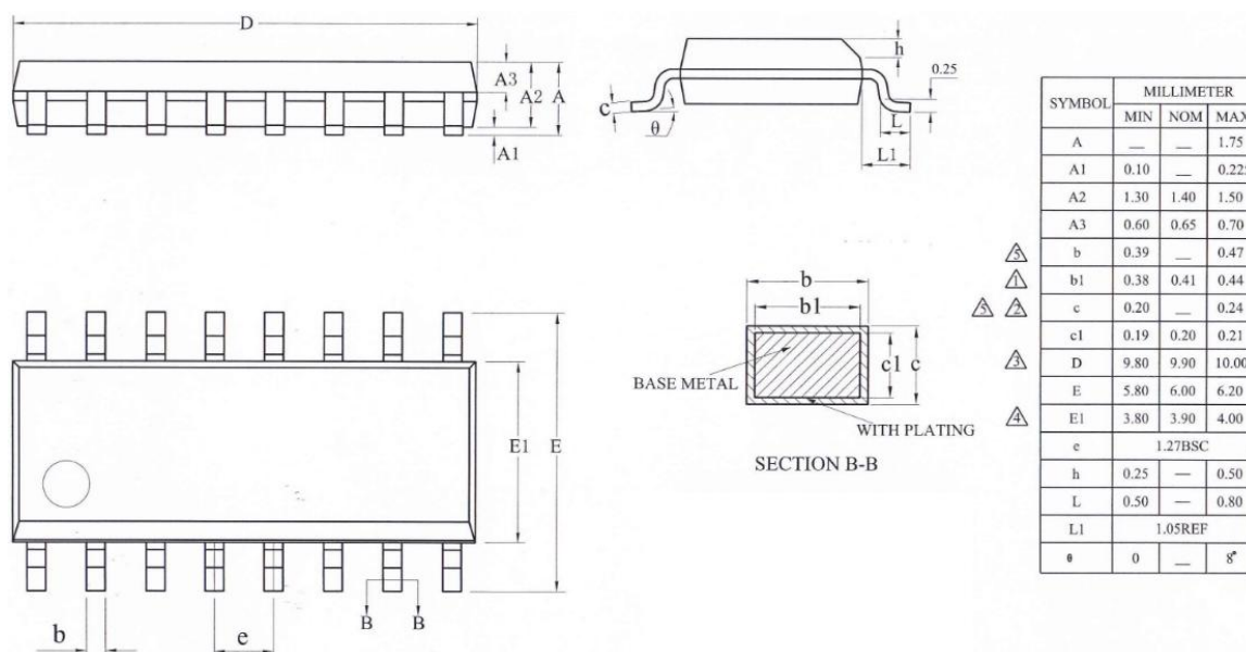
Figure 21-6 SOP16 封装尺寸
