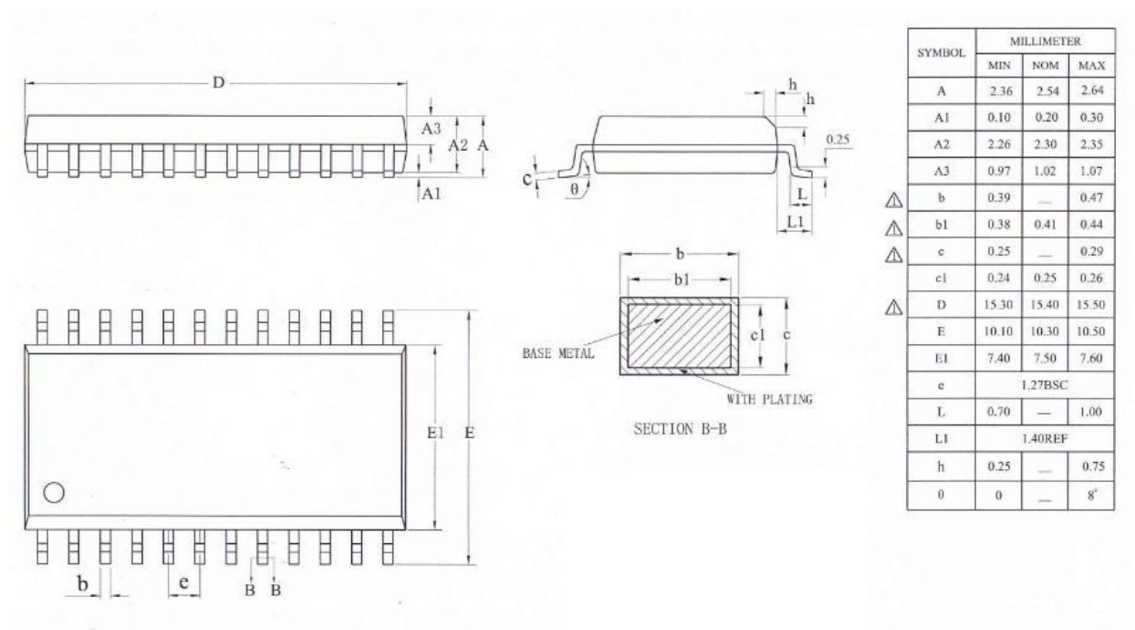
Figure 21-3 SOP24 封装尺寸
