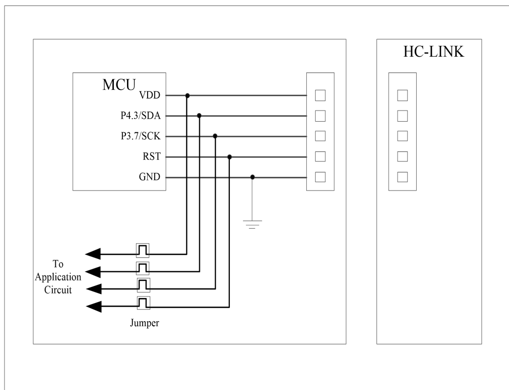
Figure 3-2 HC-LINK 编程硬件连接
