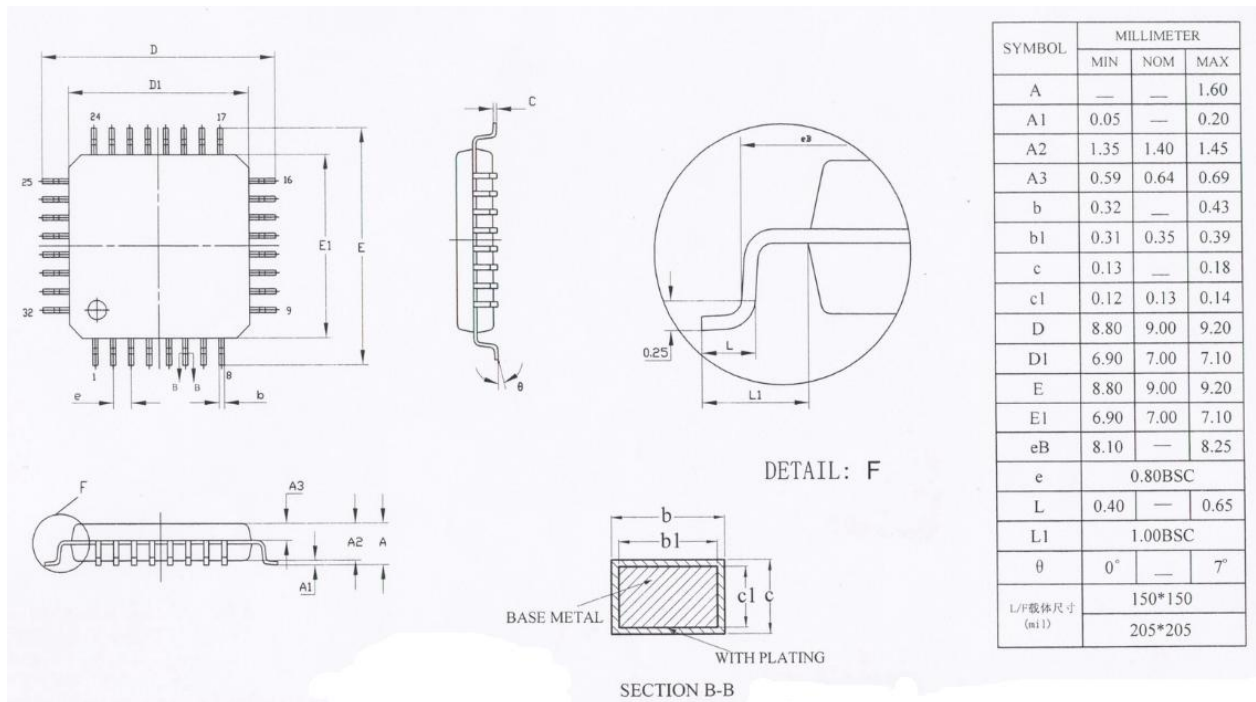
Figure 26-3 LQFP32 封装尺寸
