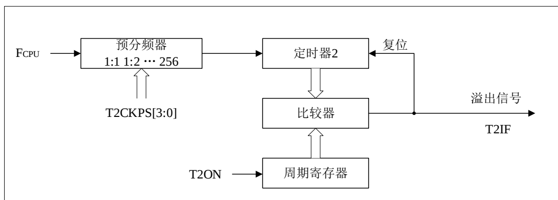
Figure 9-4 TIMER2 系统框图
