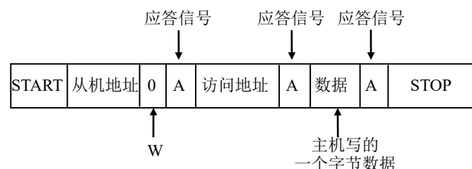
Figure 13-7 主机向从机写数据
