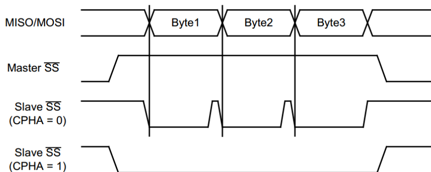
Figure 12-5 CPHA/SS 时序
