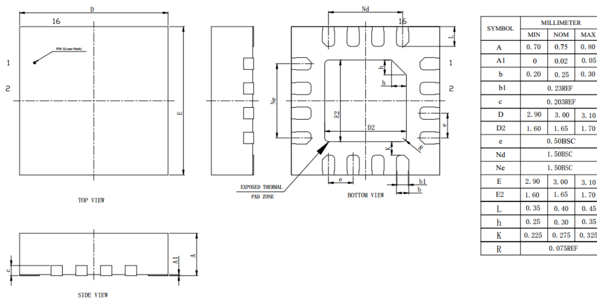
Figure 18-1 QFN16(3*3)封装尺寸
